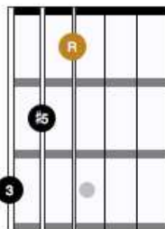
1st inversion
