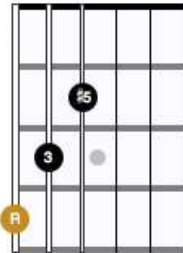
root position
